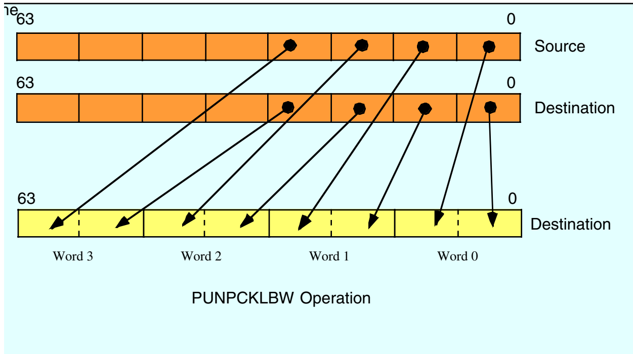
Figure 11.5 UNPCKLBW Instruction
