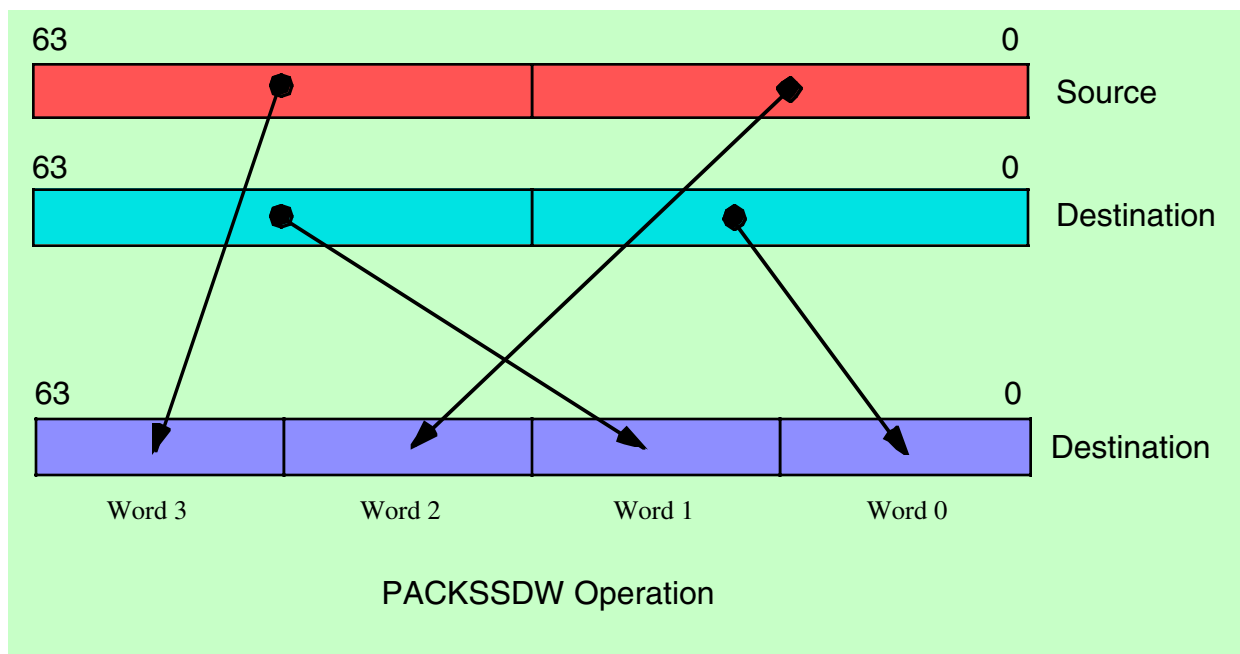
Figure 11.3 PACKSSDW Instruction
