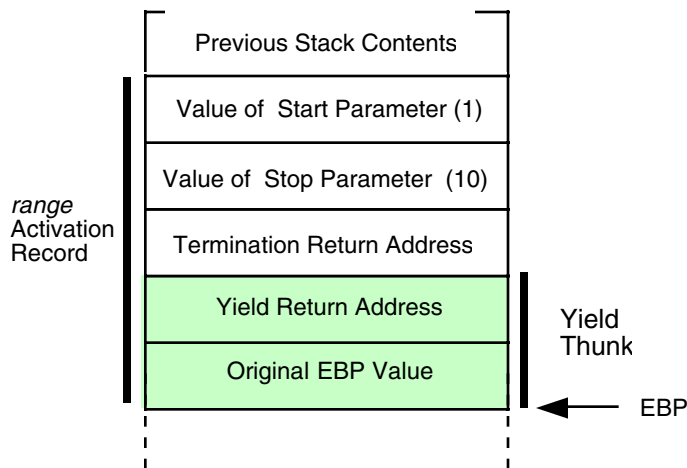
Figure 2.4 Yield Think in the range Iterator's Activation Record
